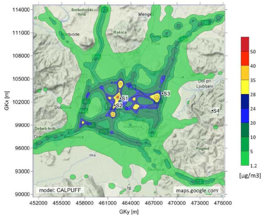
Figure 3: Preliminary results of air quality modelling (2013): the figure shows the estimated impact of road traffic pollution on annual PM 10 pollution.
